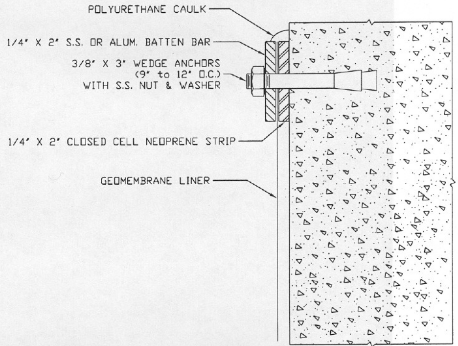
VERTICAL MECHANICAL ATTACHMENT DETAIL (Secondary Containment / Above Waterline)
