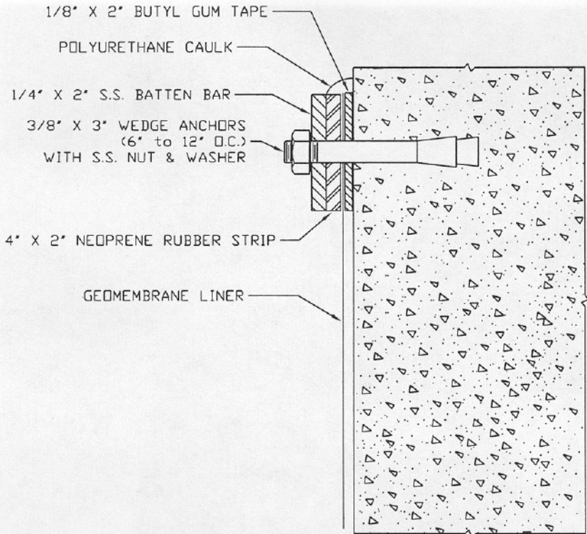
VERTICAL MECHANICAL ATTACHMENT DETAIL (Below Water)
